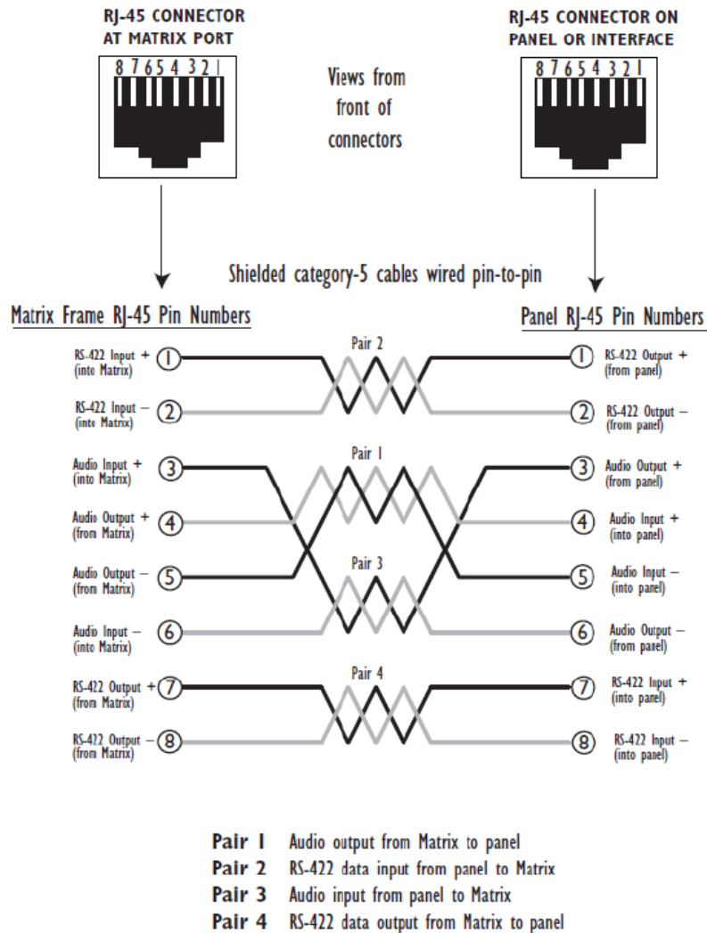
Figure 4: Connecting the matrix frame to an analog panel (4-Pair connection)
