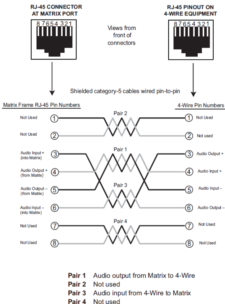
Figure 5: Connecting the matrix frame to a four-wire device (2-Pair analog)
