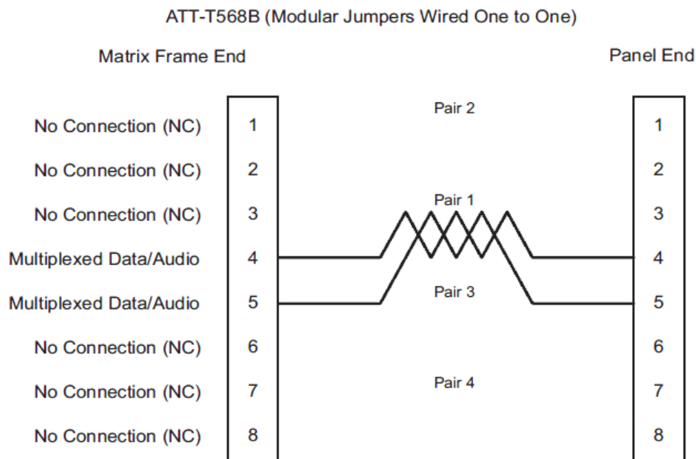
Figure 6: Connecting the matrix frame to a digital panel (single-pair digital)
