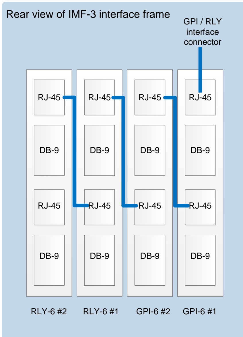
Figure 11: RLY-6/GPI-6Daisy Chain Connection
