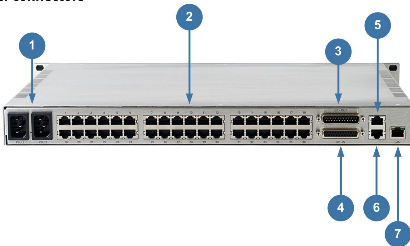
Figure 3: Rear panel connectors
